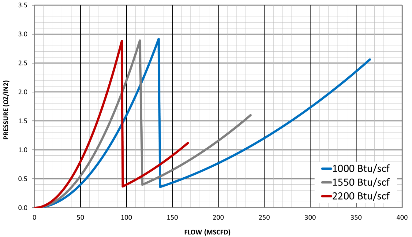
Capacity Flow Curve Model CH6030 (3rd Party Certification Pending EPA Approval)
