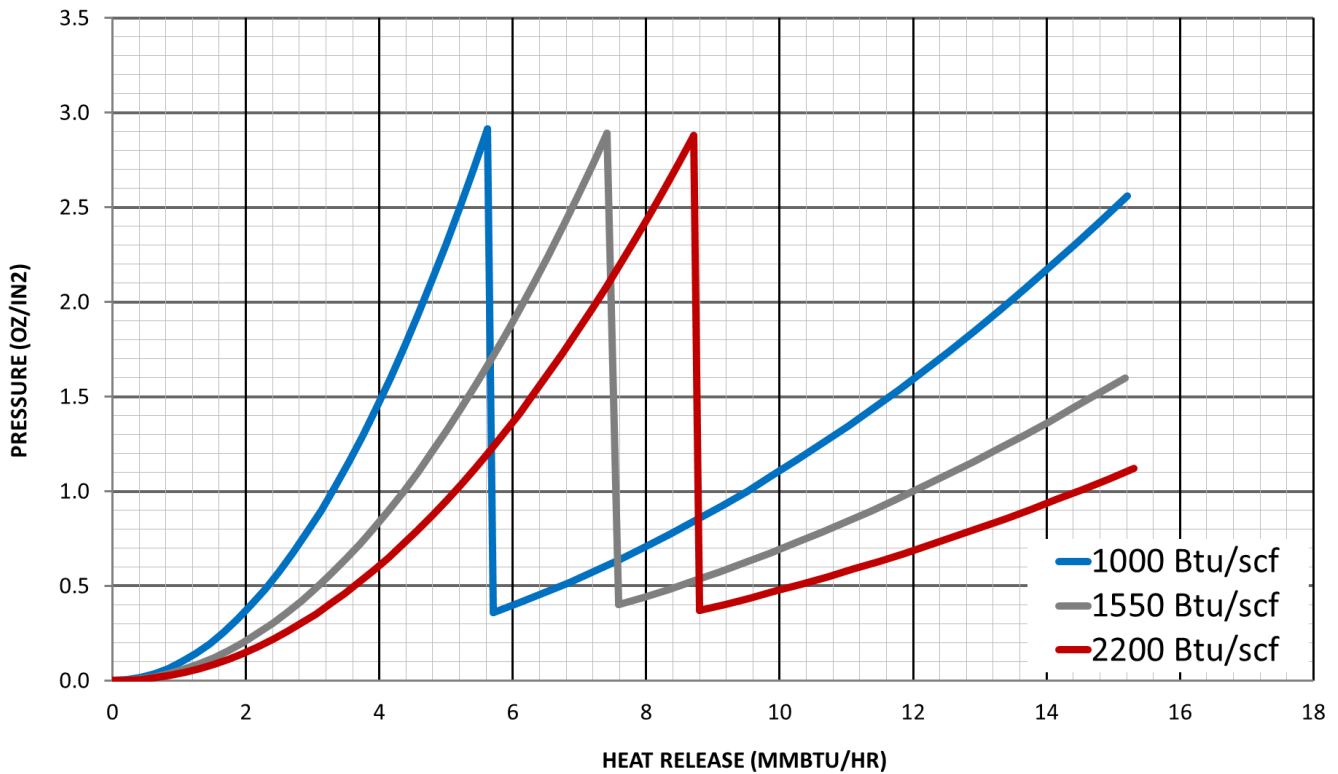
Heat Release Curve Model CH6030 (3rd Party Certification Pending EPA Approval)
